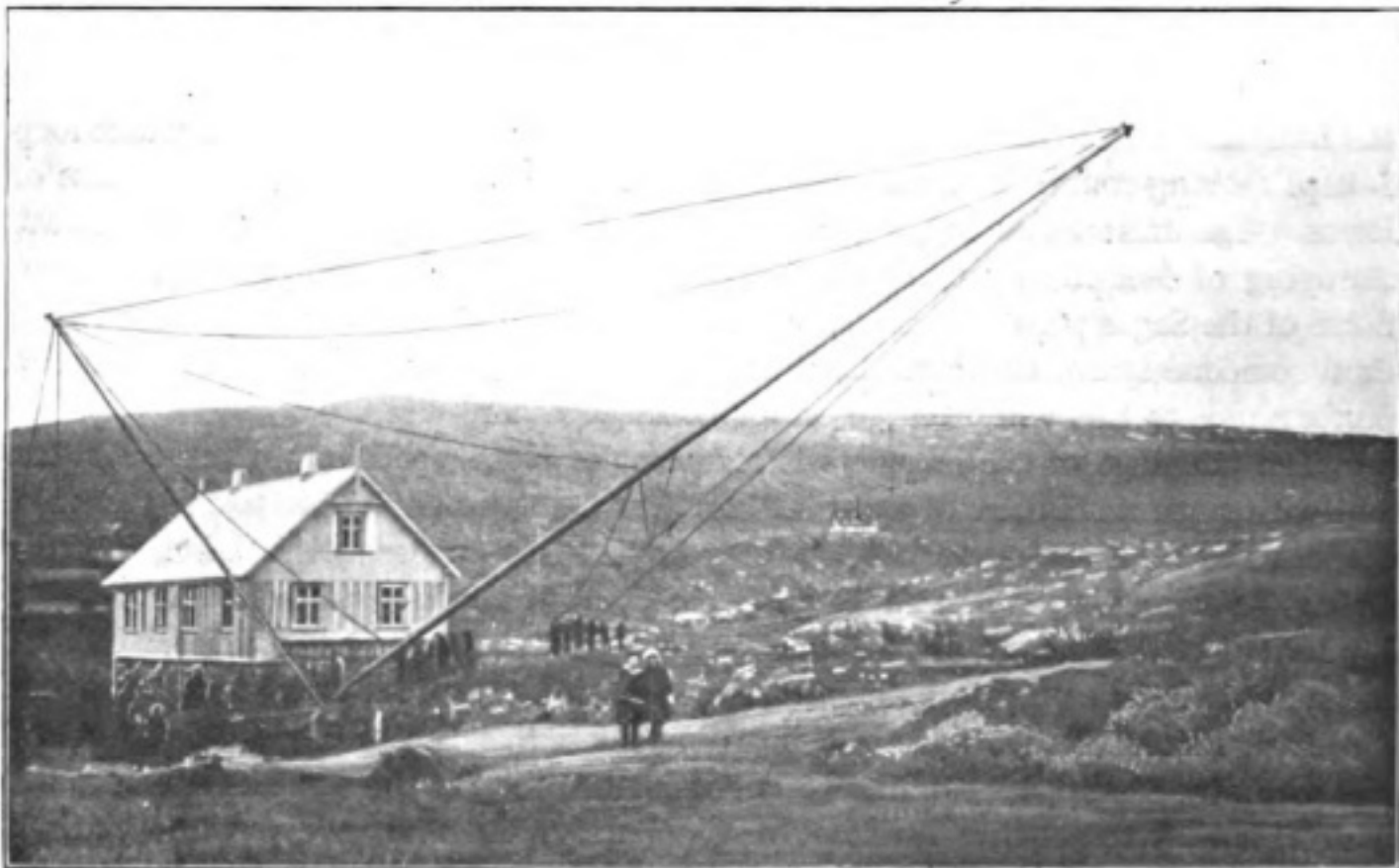
VIEW AT THORSHAVN, SHOWING THE ERECTION OF THE WIRELESS MAST BY FALLING DERRICK.
