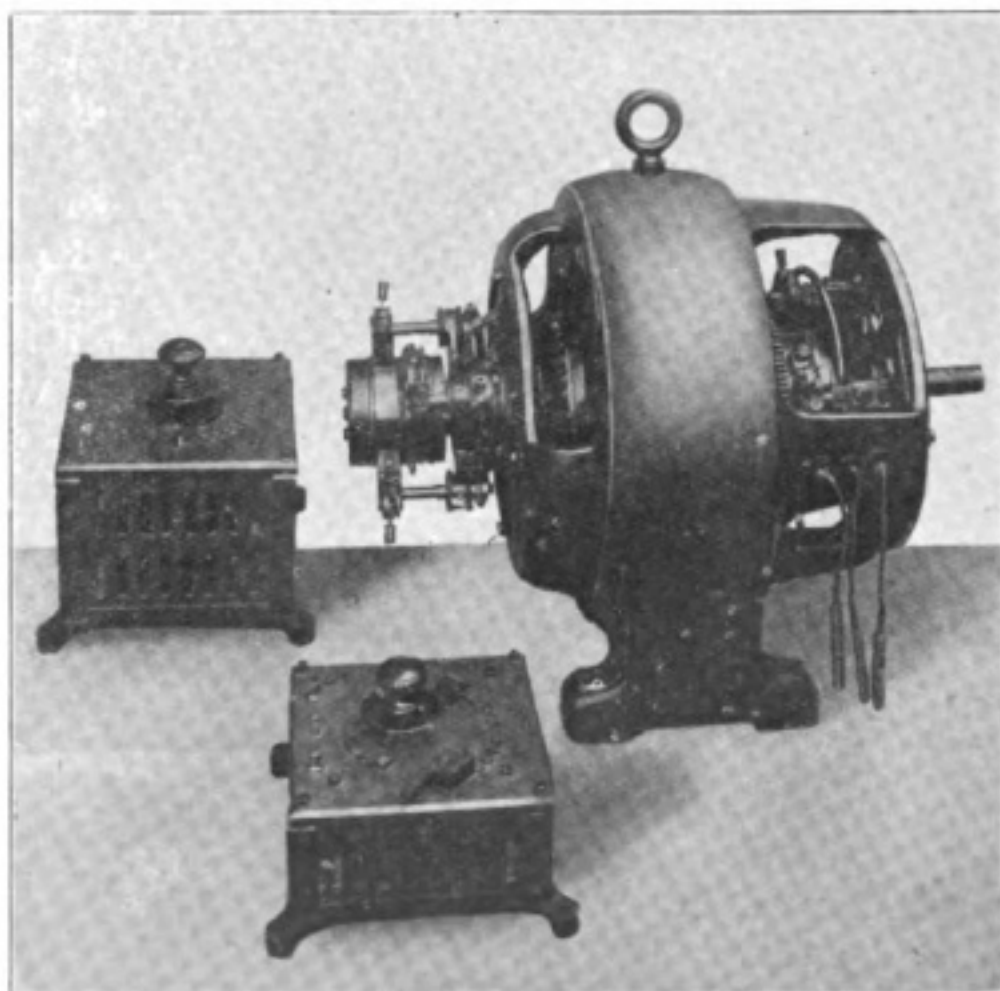
1 1/2 K.W. ROTARY CONVERTER.
